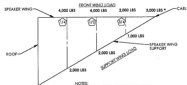
SPEAKER WING LOAD CHART
